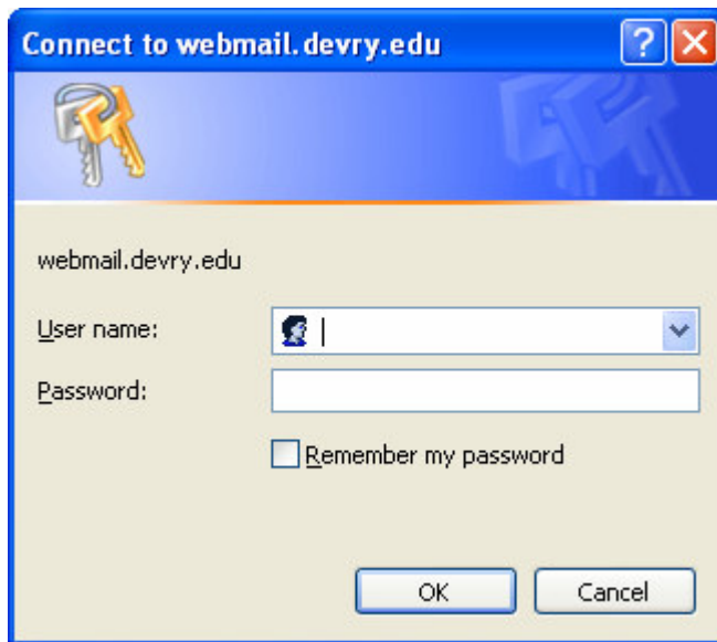
Login Window
